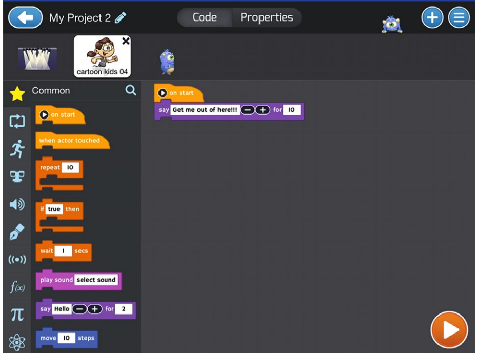
Figure 5 Tynker Interface and Coding Commands
